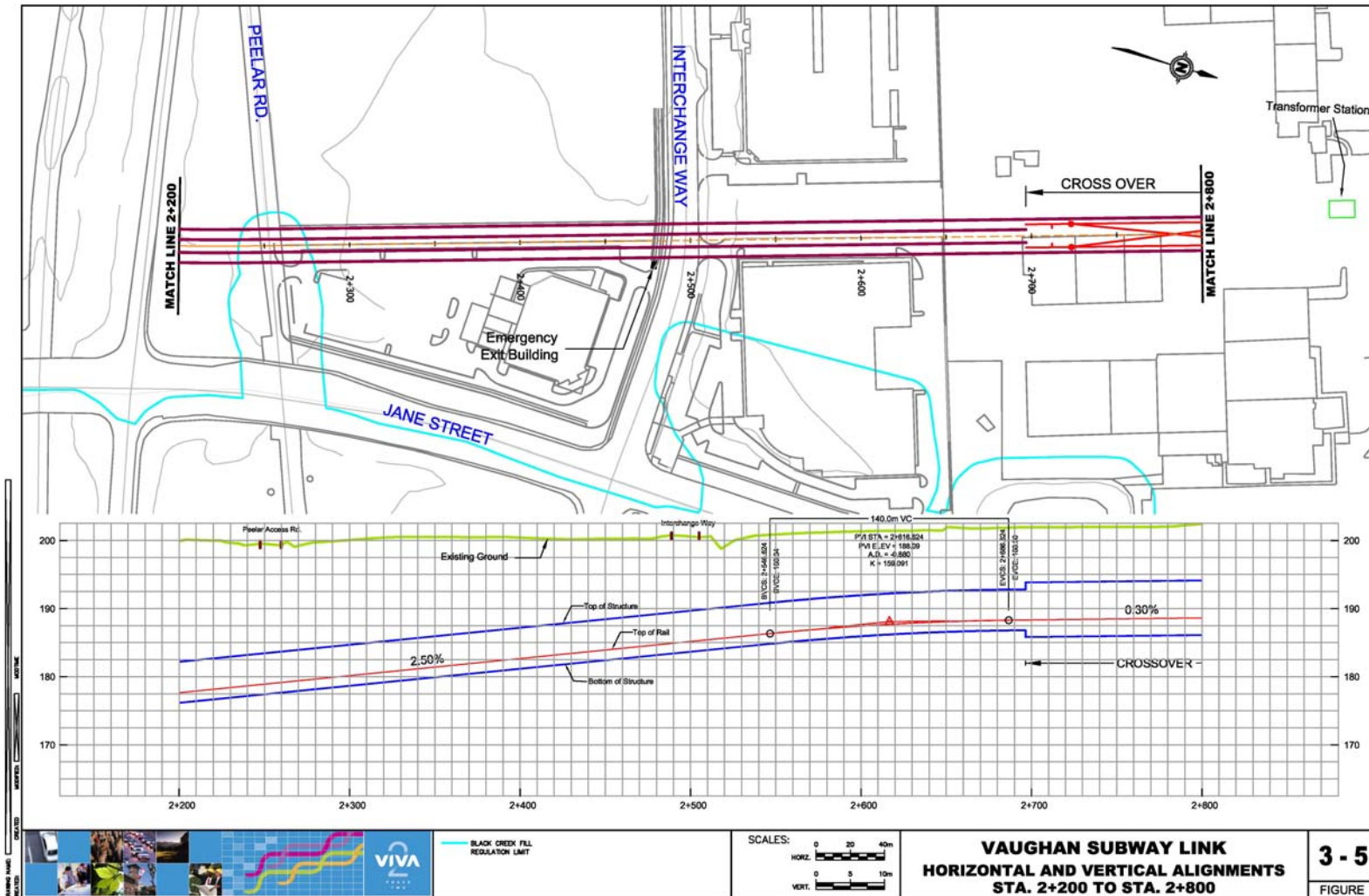
COA Report Approved Vertical and Horizontal Alignments – STA. 2 + 200 to 2 + 800 (Source: COA Report, 2007)
